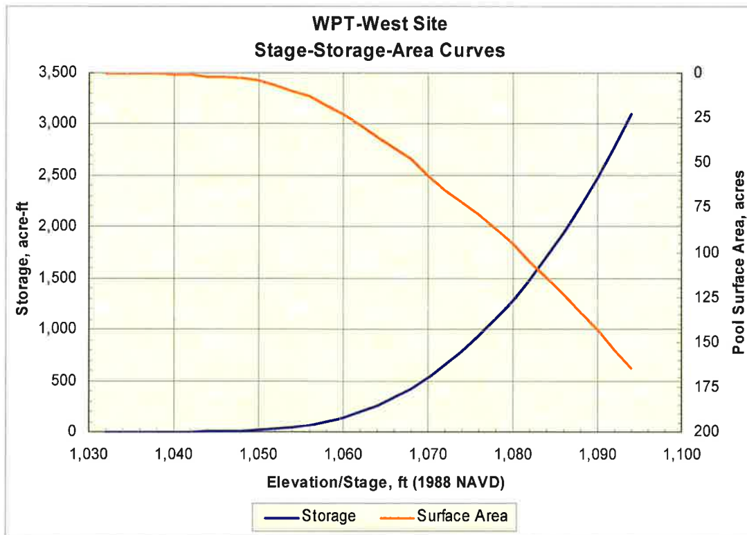
Exhibit 1 Stage-Storage-Area Curves for WPT-West Site
